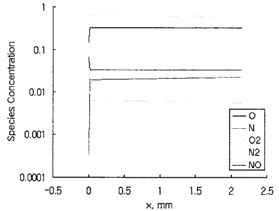
Fig. 9 Species concentration of atoms in the post shock flow region
