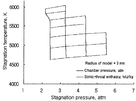
Fig. 10 Stagnation temperature distribution at the stagnation point
