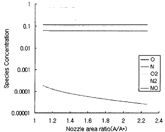
Fig. 7 Species concentration along the nozzle axis
