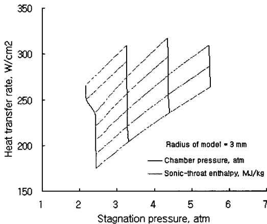
Fig. 11 Heat transfer rate at the stagnation point
