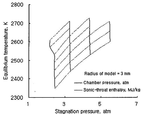
Fig. 12 Equilibrium temperature distribution at the stagnation point
