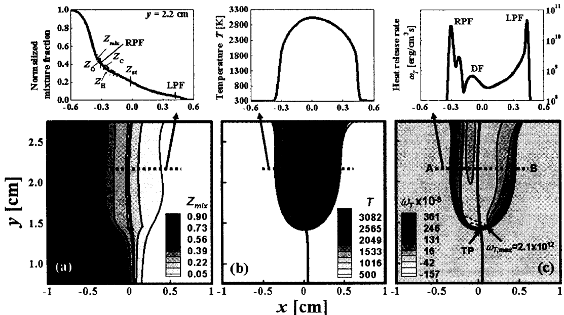
Fig. 1 Contours of the mixture fraction (a), temperature (b), and heat release rate(c) for the edge-flame snapshot at t = 0.9 ms after ignition and their horizontal profiles at the cross-section of y = 2.2 cm.
