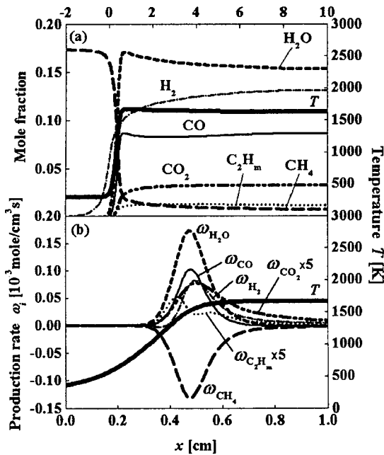
Fig. 4 The profiles of the temperature and mole fractions (a) and of the production rates (b) for \text{CH}_4 , \text{C}_2\text{H}_m , \text{CO} , \text{H}_2 , \text{CO}_2 and \text{H}_2\text{O} of 1-D \text{CH}_4/\text{air} premixed flame at \phi = 2.0 calculated by GRI-Mech 2.11.
