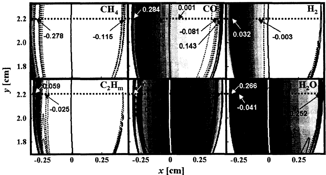
Fig. 2 The mass fraction (flood contours) and reaction rates (solid line contours: production, dotted-line contours: consumption) for CH_4 , C_2H_m , CO , H_2 , CO_2 and H_2O in the downstream diffusion-flame region.
