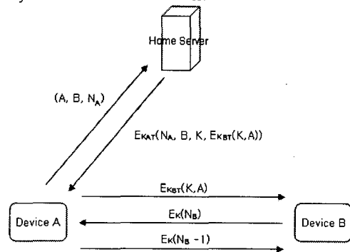
Fig 2. A interacts with a home server T and B
