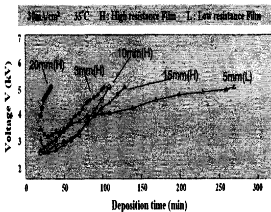
Fig. 1. Electrode distance and voltage change with deposition time.
