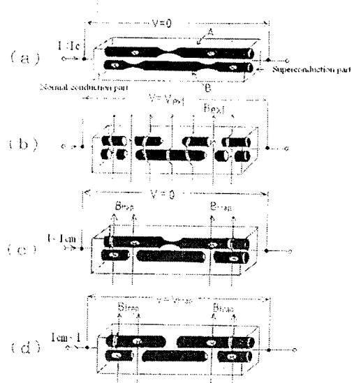
Fig. 2. Filament voltage occurrence model.
