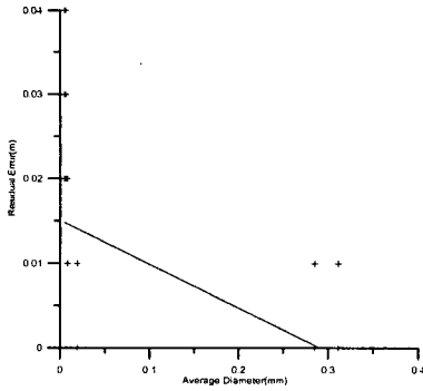
Fig. 6. Result of Linear Regression Analysis
