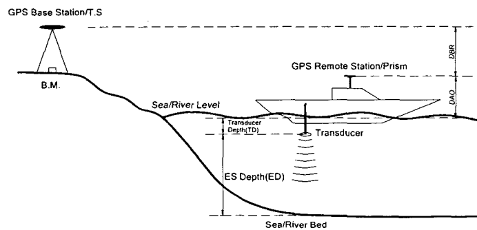
Fig. 1. Schematic of Depth Survey by Formula (1)
