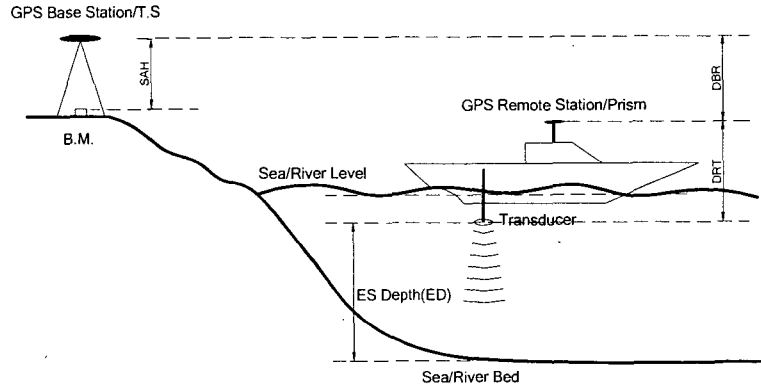
Fig. 2. Schematic of Depth Survey by Formula (2)
