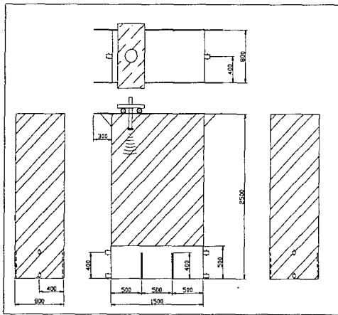
Fig. 4. Diagram of Water Tank
