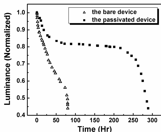
Figure 6. Lifetime of OLED with and without the passivation layer (current density was 15\text{mA}/\text{cm}^2 at room temperature).
