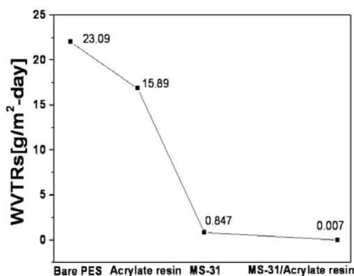
Figure 2. The WVTRs of the bare PES, Acrylate resin film, MS-31 film and the MS-31/Acrylate resin films.
