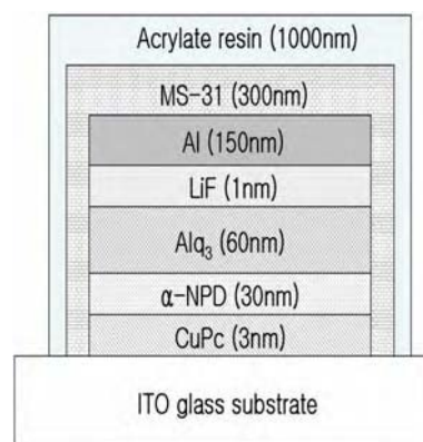
Figure 1. Schematic diagram of OLED with HTF passivation layer.
