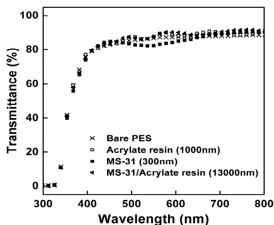
Figure 4. Transmittances of the bare PES, Acrylate resin film on PES, MS-31 film on PES and MS-31/Acrylate resin films on PES.
