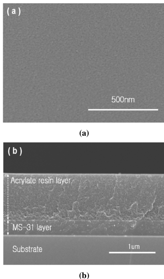
Figure 3. FE-SEM images of (a) the MS-31 surface (b) the HTF cross-section.
