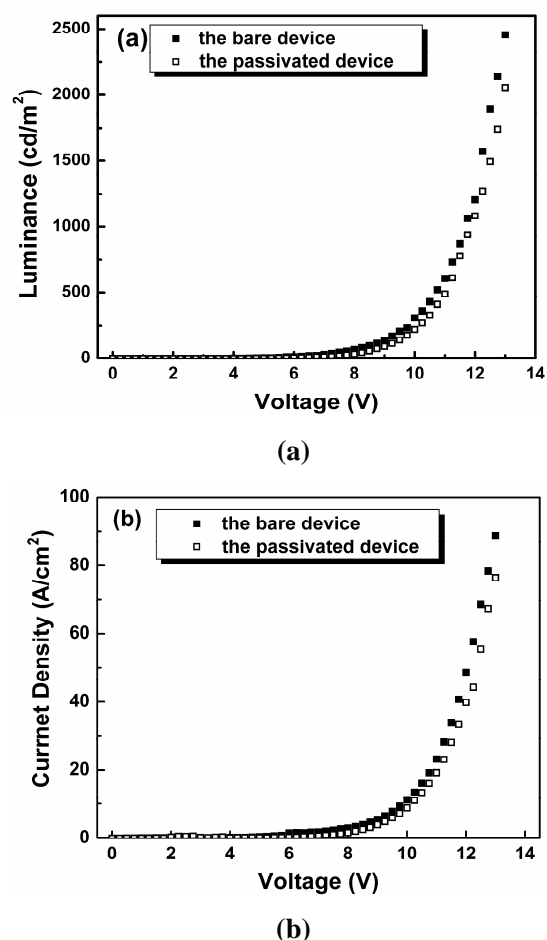
Figure 5. (a) Luminance-voltage and (b) Current-voltage characteristics of OLED.
