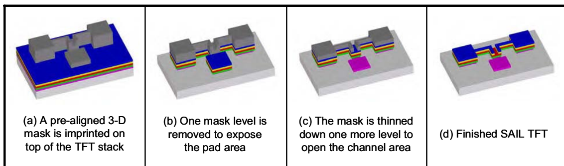
Figure 4. Schematic diagrams illustrating a process flow for SAIL TFT fabrication
