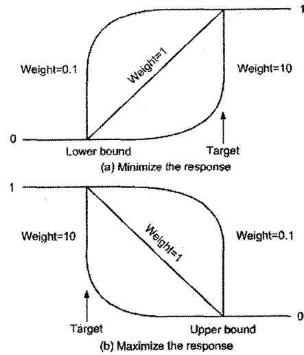
Fig. 10 Desirability function for response optimization
