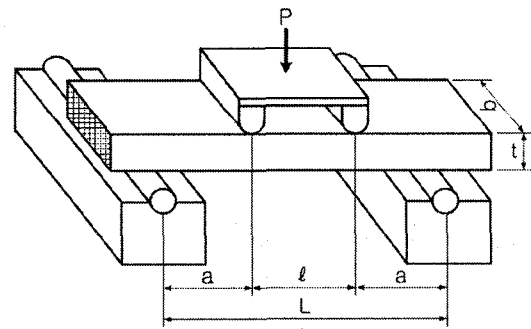
Fig. 3 Pertinent parameters for computing specimen strength during 4-point bend test
