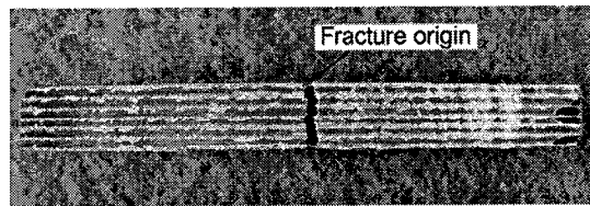
Fig. 5 Fracture pattern of axial MOR specimens
