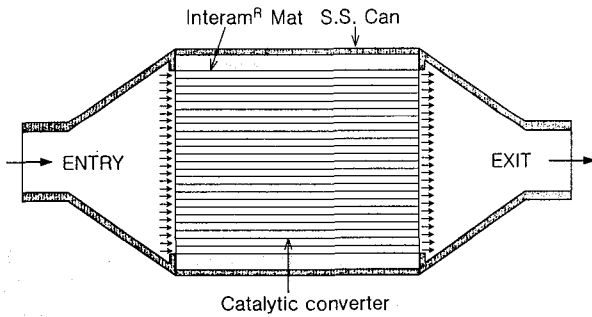
Fig. 1 Schematic of three-way catalytic converter assembly
