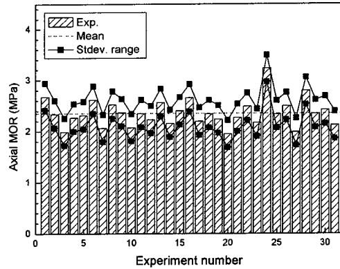
Fig. 4 Experiment results for axial MOR
