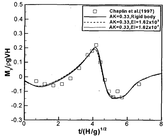
Fig. 11 Comparison of bending moment between EI = 1.62 \times 10^3 \text{ N-m}^2 and EI = 1.62 \times 10^4 \text{ N-m}^2 when A_T K_C = 0.33
