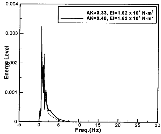
Fig. 6 Comparative spectral analysis of hydroelastic response of the vertical cylinder between A_T K_C=0.33 and A_T K_C=0.40 when EI=1.62 \times 10^4 \text{ N-m}^2
