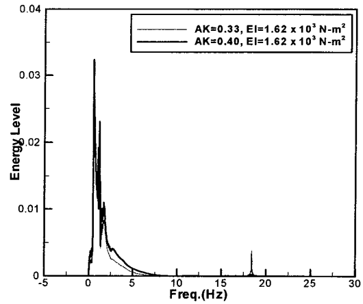
Fig. 5 Comparative spectral analysis of hydroelastic response of the vertical cylinder between A_T K_C=0.33 and A_T K_C=0.40 when EI=1.62 \times 10^3 \text{ N-m}^2
