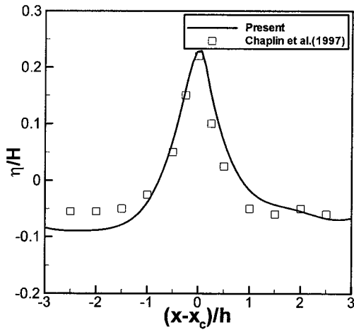
Fig. 2 Spatial distribution of wave elevation around focusing point without vertical cylinder
