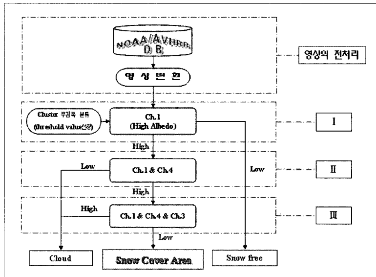
<Fig. 2> Algorithm of classification snow cover area
