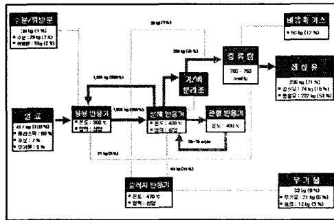
Fig. 3 Mass balance of demonstration plant
