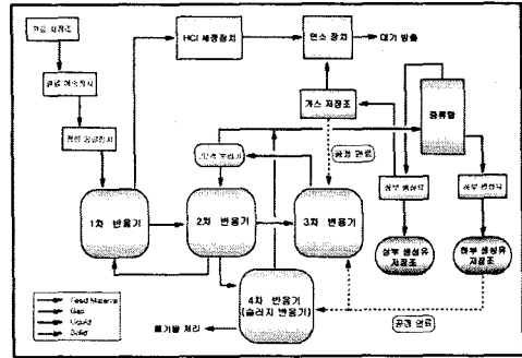
Fig. 1. Process description of demonstration plant
