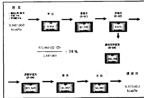
Fig. 4 Energy consumption of demonstration plant
