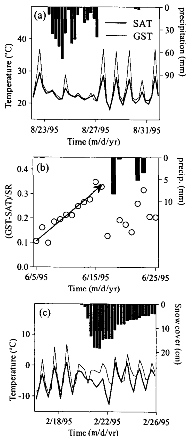
Fig. 2. Variations of GST as affected by (a) precipitation, (b) soil water content, and (c) snow cover.
