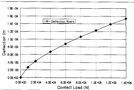
Fig. 3 Stiffness curve of Yaw Bearing
