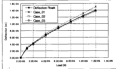
Fig. 7 Comparison of Roark's formula and FE Analysis
