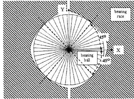
Fig. 4 Initial contact position of Yaw Bearing
