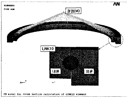
(b) FE model 02
