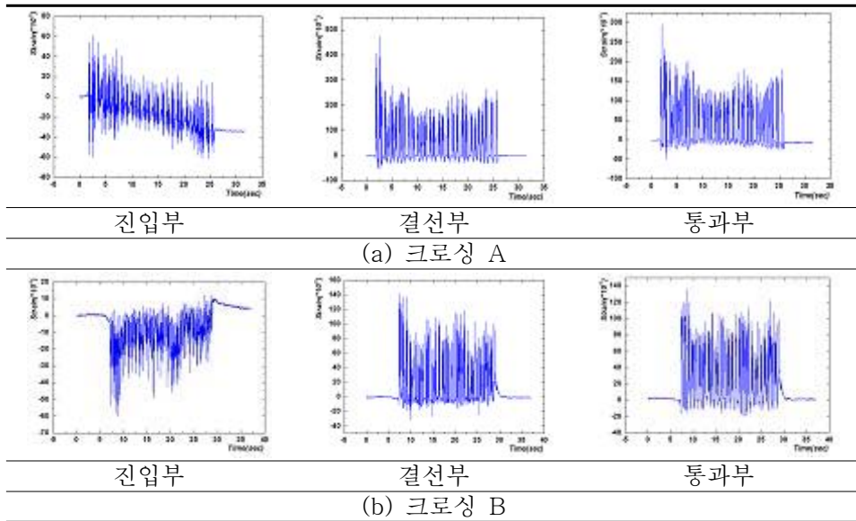
Fig 3. Test results of dynamic(strain)
