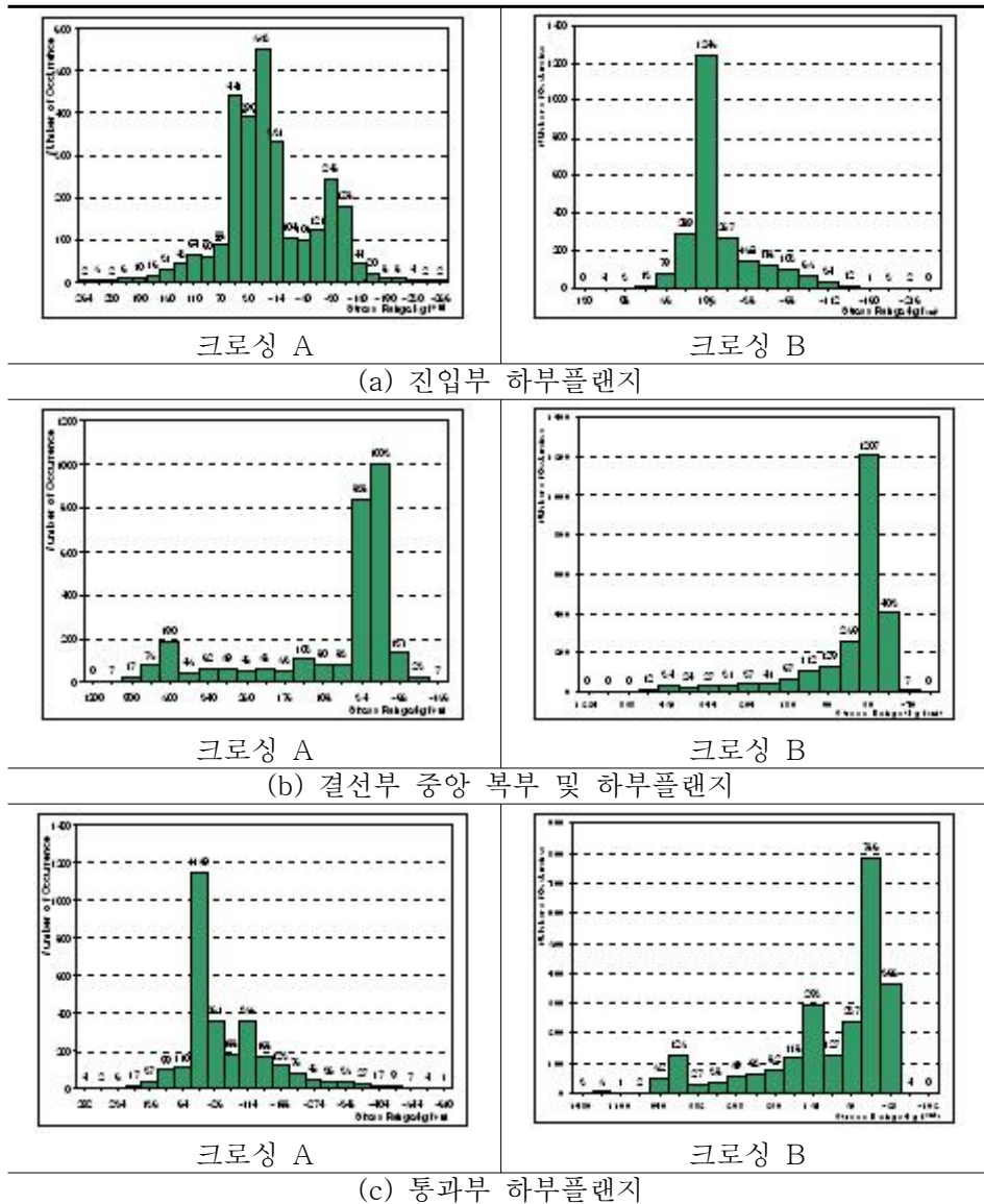
Fig 4. Stress frequency histogram
