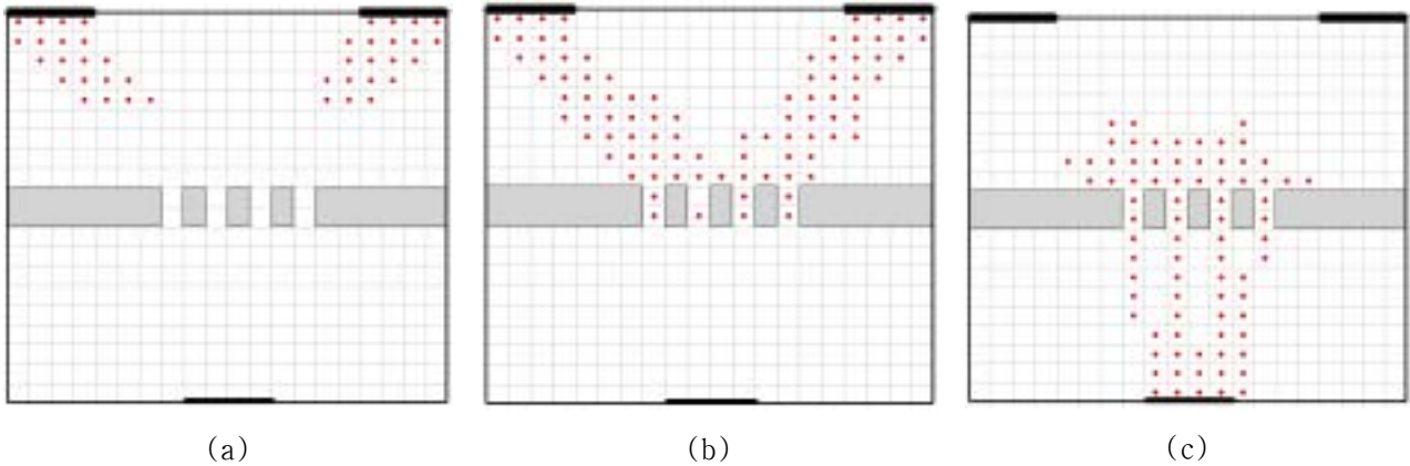
Fig.9. Simulation Results C (a)5sec, (b)10sec, (c)20sec
