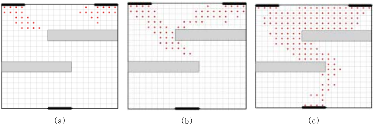
Fig.8. Simulation Results B (a)5sec, (b)10sec, (c)20sec
