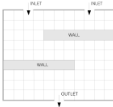
Fig.5. Simplified Model B
