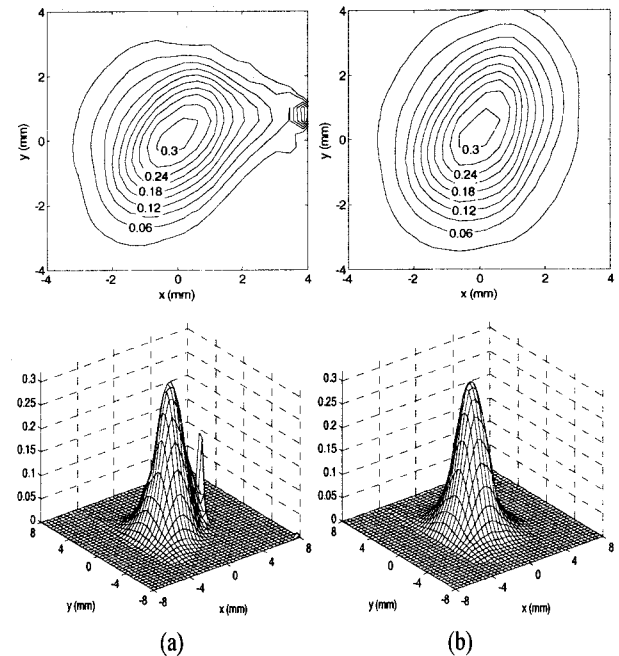
Fig. 3 Comparison of contours of reconstructed density distribution of butane flow for (a) without new integration method and (b) with new integration method
