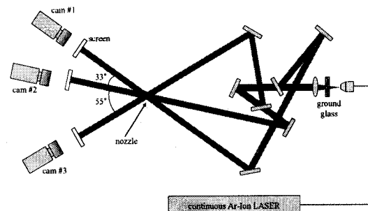
Fig. 2 Schematic diagram of digital speckle system for downward butane flow
