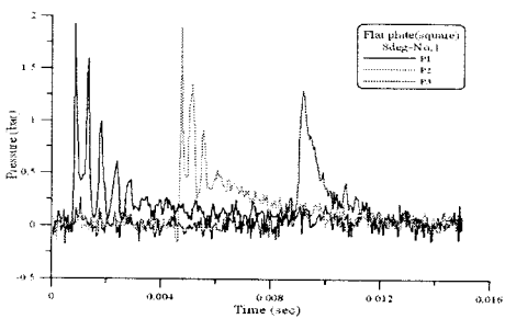
Fig. 9 Time history of pressure (8° incident angle, drop height 250mm, air pressure in the compressor 8bar)
