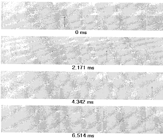
Fig. 13 Jet spray at 4°
