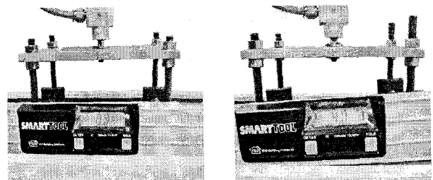
Fig. 7 Incident angles of plate setup
