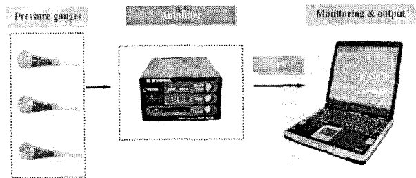
Fig. 3 Data acquisition system
