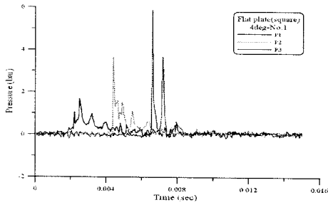
Fig. 9 Time history of pressure (4° incident angle, drop height 250mm, air pressure in the compressor 8bar)
