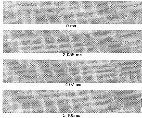
Fig. 14 Jet spray at 8°
