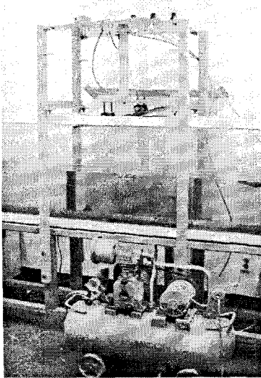
Fig. 1 Photo of Wave Flume
