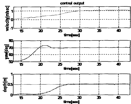
Fig. 7 PD control results - velocity, yaw and depth
