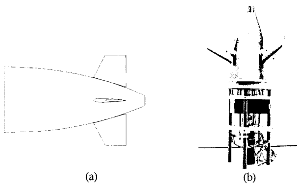
Fig. 4 Dimension and implementation of stern plane
