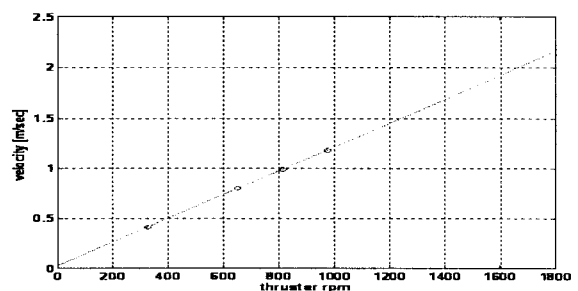
Fig. 5 Thruster rpm vs. advance speed of ISiMI
