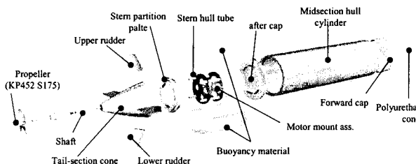
Fig. 3 Conceptual view of hull structure of ISiMI
