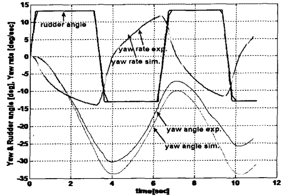
Fig. 6 Open loop zig-zag test results compared with simulation
