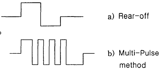
Fig.2 Write compensation method
