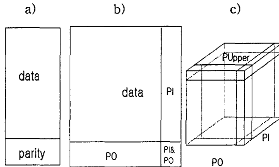
Fig.5 Data correction structure a) MOD 5(or 10) way RS(120,104) b) DVD Reed Solomon Product Code(RSPC) of RS(208,192) x RS(182,172) c) Example RS cube code RS(104,100) x RS(104,100) x RS(104,100). Data Correction structure requirements are 1. Size of data correction structure should be less than a revolution. 2. High correction performance with relatively low parity rate. 3. Interleaving to divide defect error to a lot of code-words.
