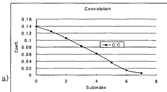
Fig.3 double sampled binary data and their convolution. C_k = \sum_{i=-n}^n b_i D_{k+i} a) convolution coefficients. b) emulated HF signal by the diffraction limited optical system
