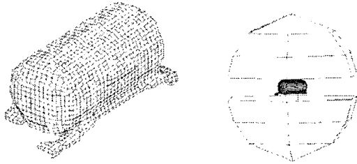
Fig 7. Acoustic mesh and Field point mesh
