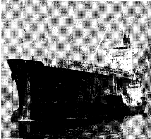
Cargo Loading from Small LPG Tanker (Ship-to-ship transfer at sea)
