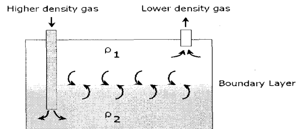
Piston Effect
