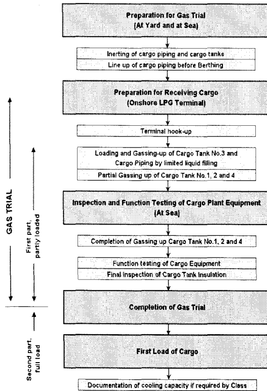
Gas Trial Flow Chart (typical)
