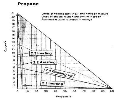
Flammability Diagram
