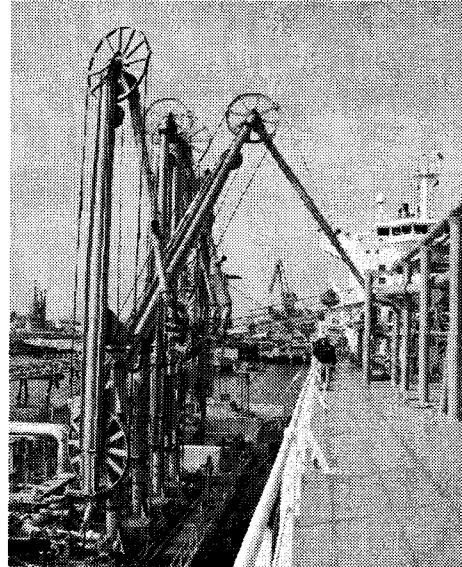
Cargo Loading from Terminal (Cargo vapor to be returned to shore)
