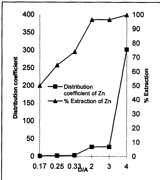
[Aq. Feed= 0.31 g/L Zn Time=5 minute, Temp. 25 °C] Figure-5: Effect of O/A ratio on the extraction of zinc using 5% Cyanex 302
