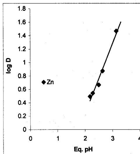
Figure-8 : Graph of log D Vs. equilibrium pH
