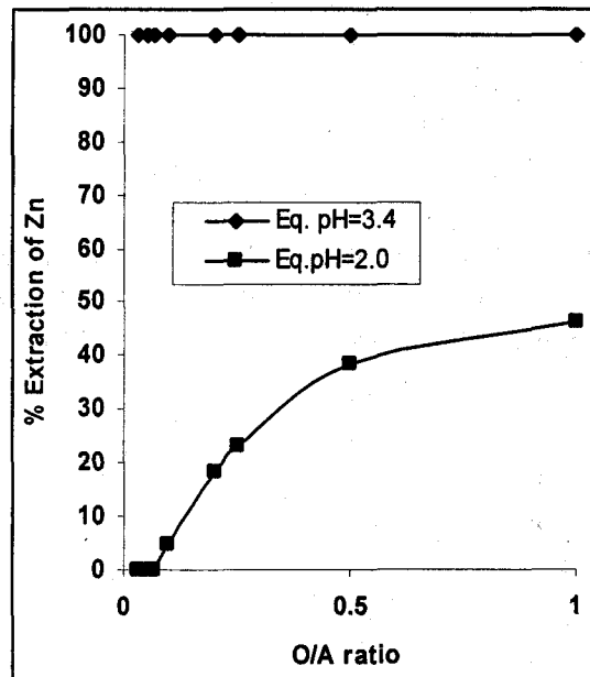
[Aq. Feed=0.085 g/L Zn and 0.025 g/L Ca, Time=5 minute, Eq. pH=3.4 Temp. 25 °C] Figure- 10 : Extraction of zinc from Baroda rayon effluent using 5% Cyanex 302 at different O/A ratio
