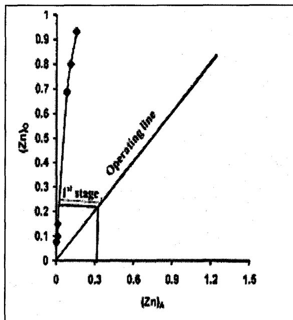
Figure-6 : Extraction isotherm of zinc from the using 5% Cyanex 302
