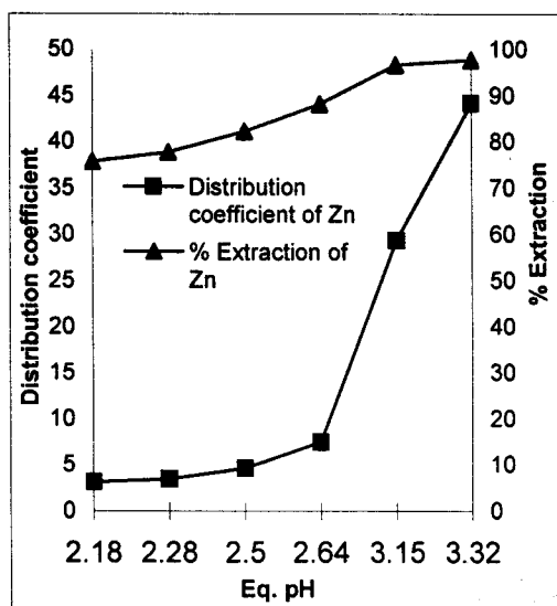
[Aq. Feed=0.085 g/L Zn and 0.025 g/L Ca, Time=5 minute, Temp. 25 °C] Figure-7: Extraction of zinc from Baroda rayon effluent using 5% Cyanex 302
