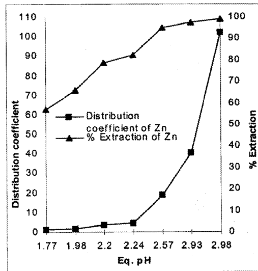
[O/A=1, Time=5 minute, Temp. 25 °C] Figure-2: Extraction of zinc from aqueous solution containing 0.46 g/L Zn using Cyanex 302.
