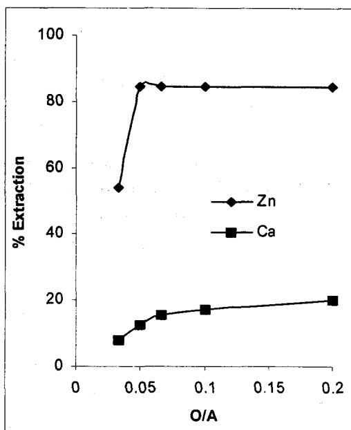
[Aq. Feed=0.085 g/L Zn and 0.025 g/L Ca, Time=5 minute, Eq. pH=3.4 Temp. 25 °C] Figure-9: Extraction of zinc from Baroda rayon effluent using 5% Cyanex 272 at different O/A ratio
