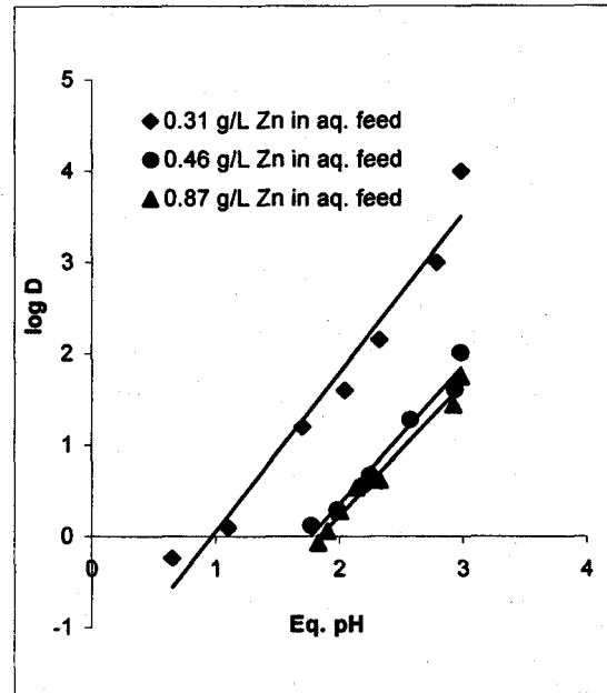
[O/A=1, Time=5 minute, Temp. 25 °C] Figure-4 : log D vs Equilibrium pH for the extraction using 5% Cyanex 302
