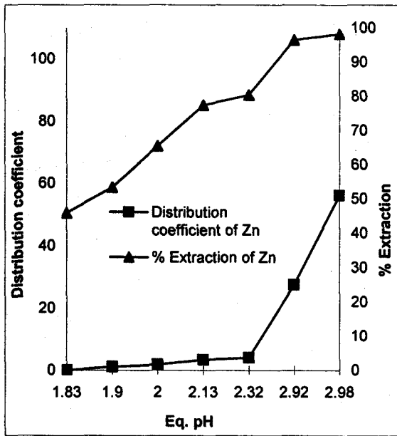
[O/A=1, Time=5 minute, Temp. 25 °C] Figure-3: Extraction of zinc from the aq. Feed of zinc containing 0.87 g/L Zn using Cyanex 302
