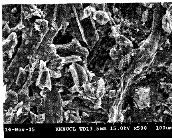
Photo 3. SEM of oak white charcoal KOCC sheet(120-140 mesh fraction, 500x).
