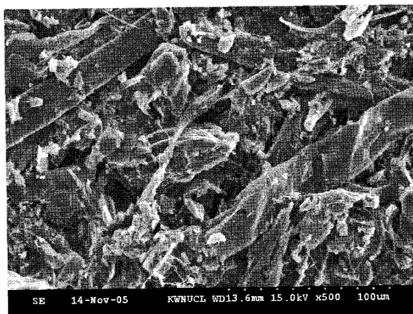
Photo 4. SEM of pine white charcoal KOCC sheet(120-140 mesh fraction, 500x).
