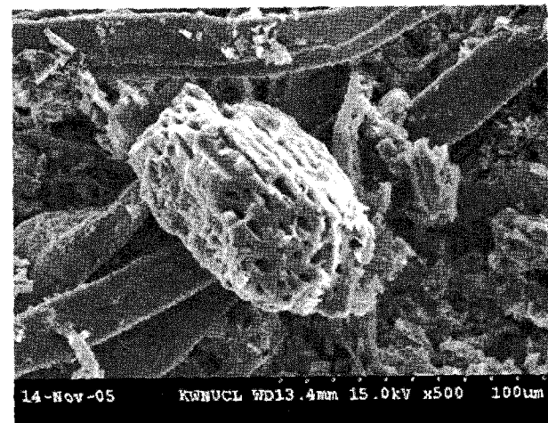
Photo 2. SEM of oak black charcoal KOCC sheet(100-120 mesh fraction, 500x).
