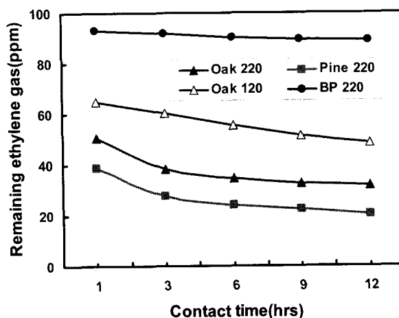
Fig. 5. Effects of species on the ethylene gas adsorption.
