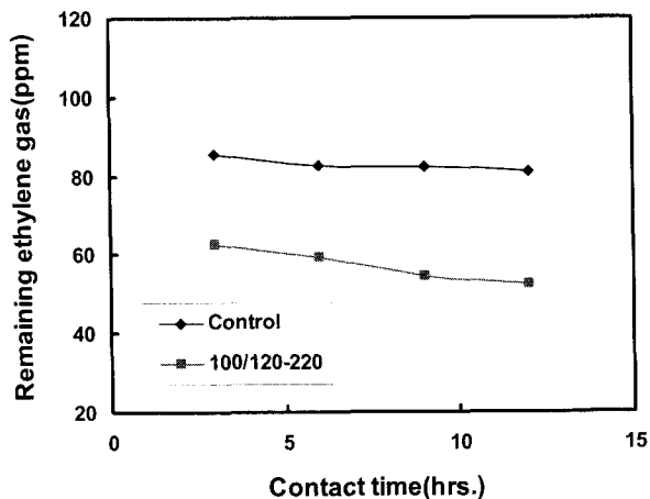
Fig. 4. Ethylene gas adsorption of ONP charcoal sheet.
