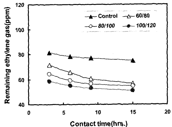
Fig. 2. Effects of particle size of black oak charcoal on the ethylene gas adsorption of KOCC charcoal sheet.
