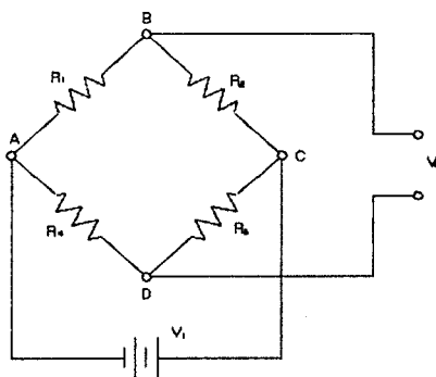
Fig. 1 Wheatstone Bridge Composition
