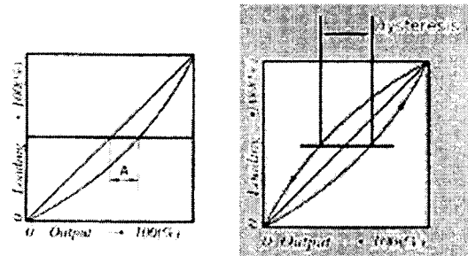
Fig. 2 Hysteresis Curved Line Output
