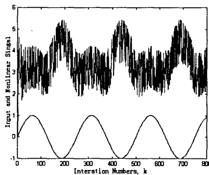
Fig.4 Plant Output of typical DNN
