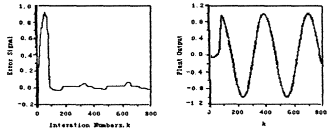
Fig.3 Error Signal of typical DNN
