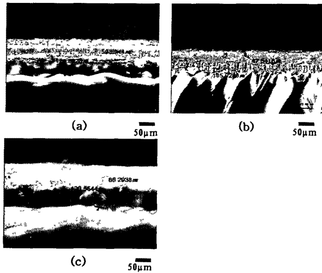
Fig. 6 Optical microscope pictures of cross-section (a) 355nm, (b) 532nm, (c) 1064nm
