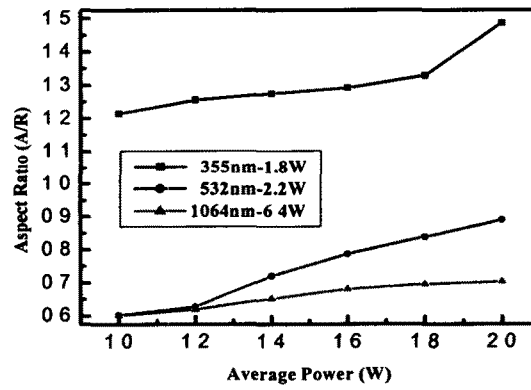
Fig. 4 Aspect ratio(A/R) with wavelength
