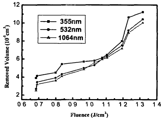
Fig. 2 Removed mass for fluence with wavelength
