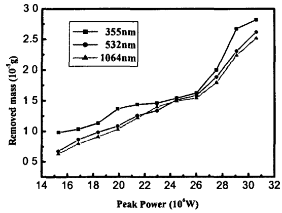
Fig. 3 Removed volume for peak power with wavelength
