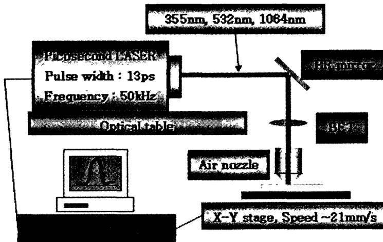
Fig. 1 Schematic illustration of experimental equipment
