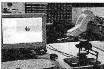
Fig.6 View of Master/Slave Control System
