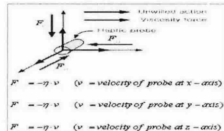
Fig.4 Algorithm of Viscosity Force
