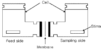
Fig. 1. Schematic diagram of permeable cell
