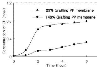
Fig. 5. Permeation of Cl -
