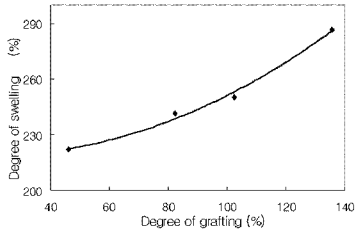
Fig. 4. Degree of swelling by degree of grafting
