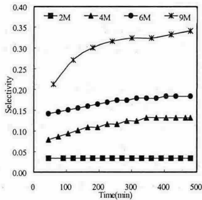
Fig 1. Effect of Feed Concentration on Selectivity of Nitric Acid.
