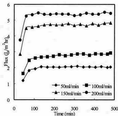
Fig 3. Effect of Feed Flow Rate on Flux of 4M Nitric Acid.
