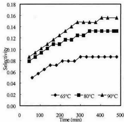
Fig 2. Effect of Feed Temperature on Selectivity of 4M Nitric Acid.
