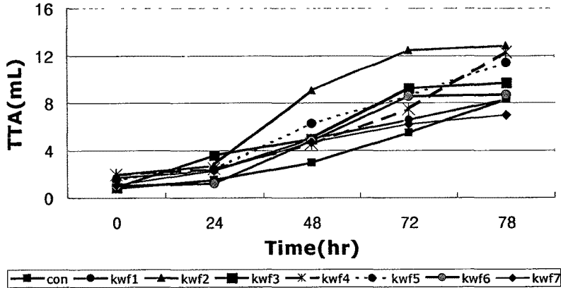
Fig. 2. TTA changes for the control and KWF sourdough starters
