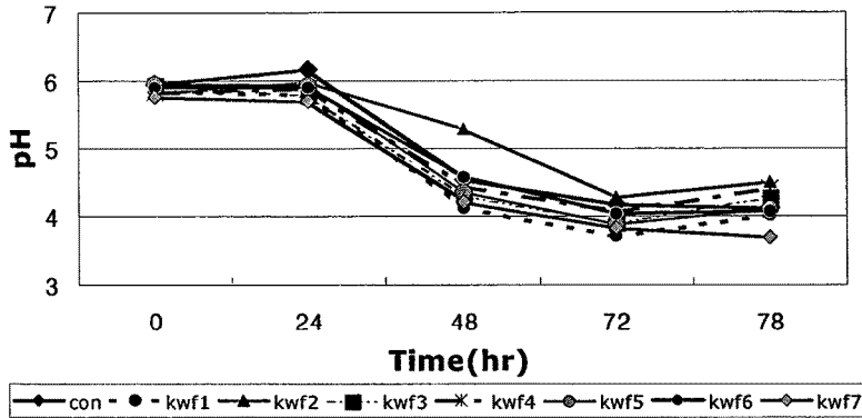
Fig. 1. pH changes for the control and KWF sourdough starters
