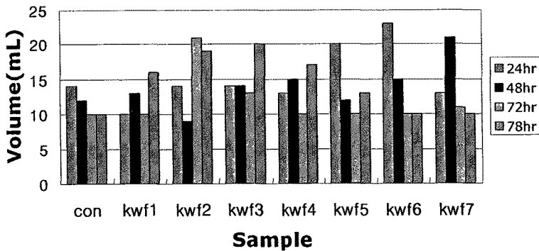
Fig. 3. Volume of sourdough starters
