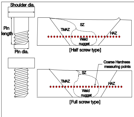
Fig. 1 Vickers hardness measuring position of welding zone on Butt-jointed specimen by pin of full screw type and half screw type
