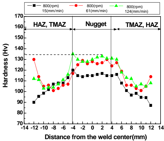
Fig. 4 Comparison of micro vickers hardness profiles on the cross-section of the welded zone according to welding conditions using pin of half screw type (shoulder dia. 20φmm; pin dia. 4φmm; pin length 6mm) and rotation speed 800rpm
