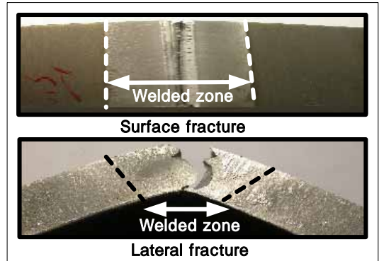
Fig. 11 Fracture surface and lateral face of the defect guided bending test specimen by FSW
