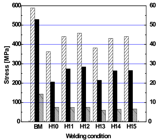
Fig. 8 Comparison of tensile stress, 0.2% offset yield point and elongation(%) of the weld joints according to the welding speeds and the transition speeds with half screw type tool of shoulder dia. 20 \phi mm, pin dia. 6 \phi mm, pin length 6mm and shoulder dia. 15 \phi mm, pin dia. 6 \phi mm, pin length 6mm.
