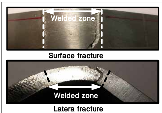
Fig. 10 Fracture surface and lateral face of the defect-free guided bending test specimen by FSW
