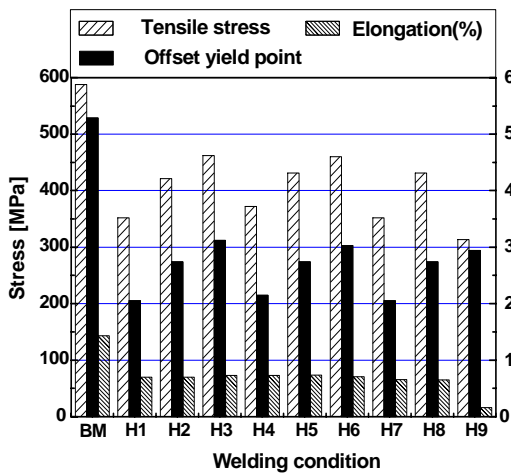
Fig. 7 Comparison of tensile stress, 0.2% offset yield point and elongation(%) of the weld joints according to the welding speeds and the transition speeds with half screw type tool of shoulder dia. 20 \phi mm, pin dia. 4 \phi mm, pin length 6mm.
