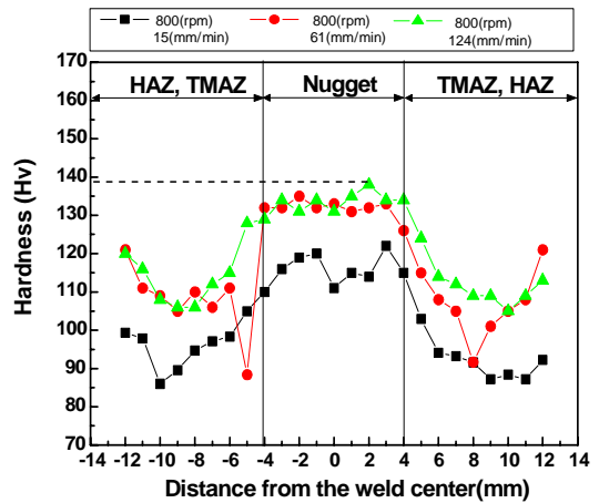
Fig. 5 Comparison of micro vickers hardness profiles on the cross-section of the welded zone according to welding conditions using pin of half screw type (shoulder dia. 15φmm; pin dia. 4φmm; pin length 6mm) and rotation speed 800rpm
