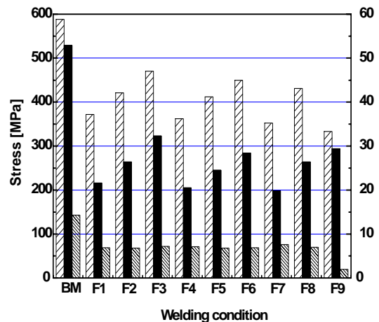
Fig. 9 Comparison of tensile stress, 0.2% offset yield point and elongation(%) of the weld joints according to the welding speeds and the transition speeds with full screw type tool of shoulder dia. 20 \phi mm, pin dia. 6 \phi mm, pin length 6mm.
