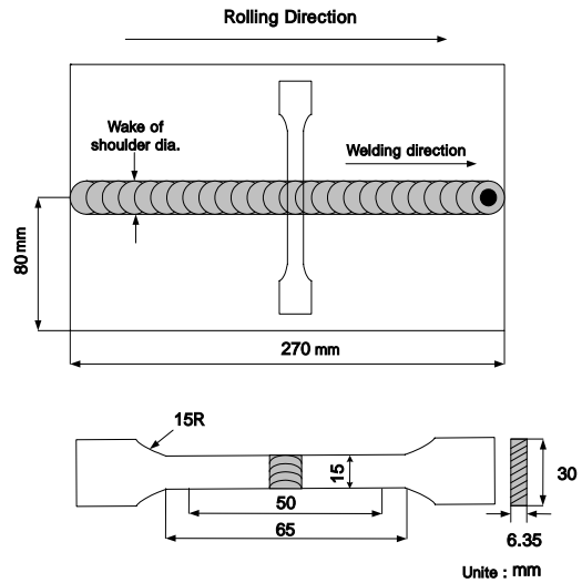
Fig. 2 Schematic of F.S Welding direction and tensile test specimens
