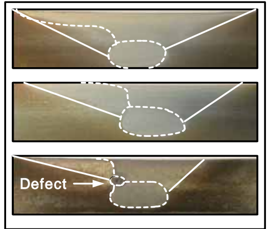
(c) Rotation speed 1600rpm
