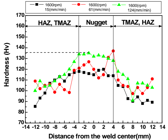
(c) Rotation speed 1600rpm
