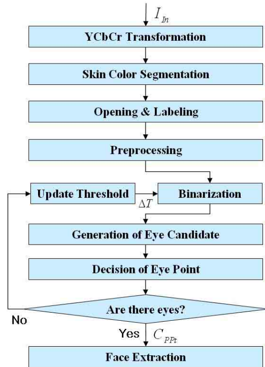
Fig. 5 The flow chart of proposed face detection system.
