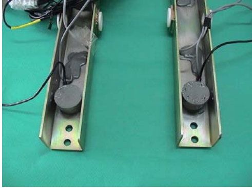
Figure 9 Accelerometers under cross beam
