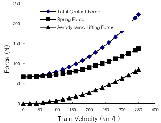
Figure 11 Analyzed forces
