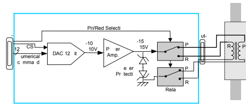
Figure 5 Circuit of driving electronics
