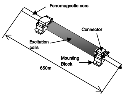
Figure 1 Structure of magnetic torquer
