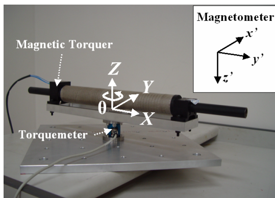
Figure 13 Coordinate definition
