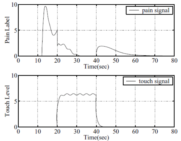
Fig. 16. Output of Neural Network: contact force 600g/m^2
