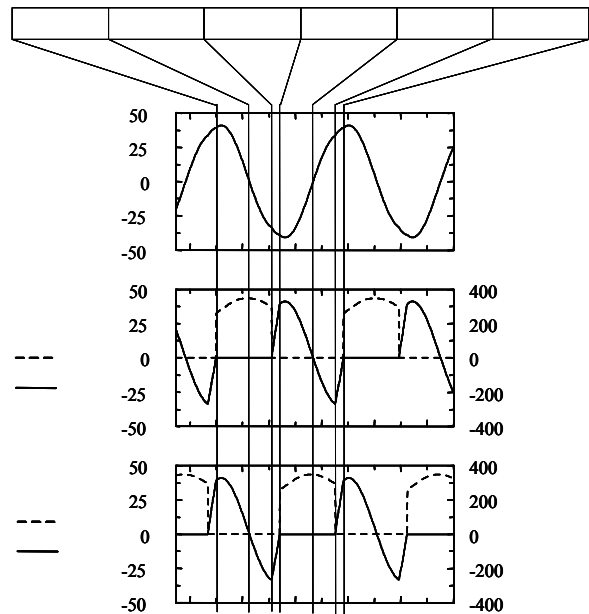
Fig.6 Voltage and current waveforms in steady state of power injection
