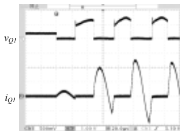
v_{Q1} :250[V/div], i_{Q1} :20[A/div], t 20[ \mu sec/div] (a) Voltage and current on Q_1
