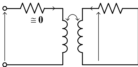
Fig.3 Transformer model of induction heating load
