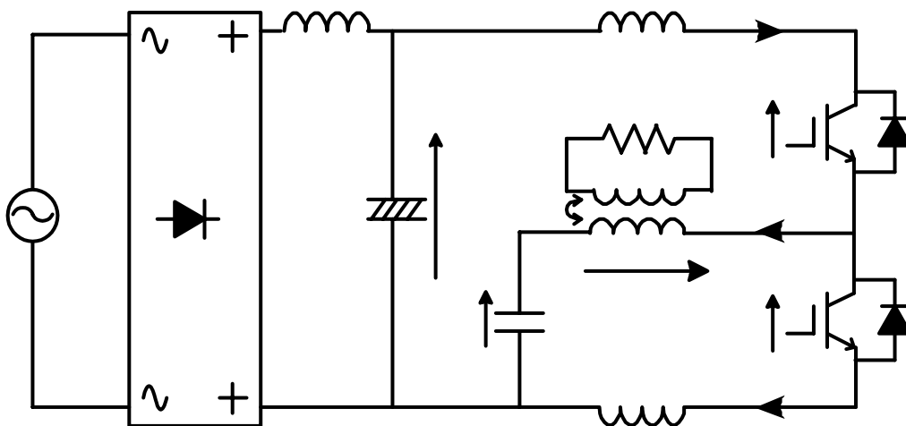
Fig.4 Voltage source SEPP ZCS-PDM high frequency inverter system for induction heated fixing roller
