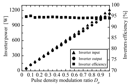
Fig.10 Power regulation characteristics in experiment
