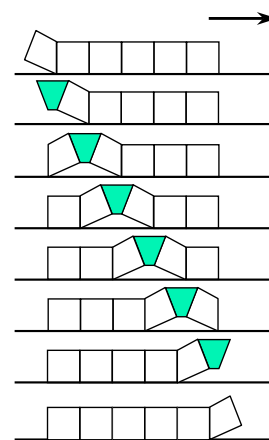
Fig. 3. Caterpillar locomotion.
