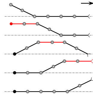
Fig. 15. 2-2-2 motion pattern of 6 link model as a combination of only two-singular links.
