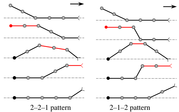
Fig. 10. Motion patterns of 5 link model as a combination of two-singular links and one link, where two-singular links motion is used twice.
