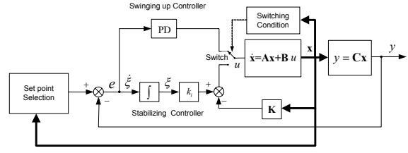
Fig. 2 Structure of the proposed control system.
