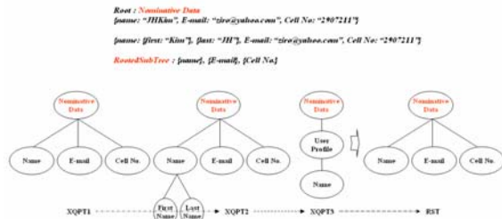
Fig. 2 XML Query Pattern Tree applied for Mining XQuery Stream
