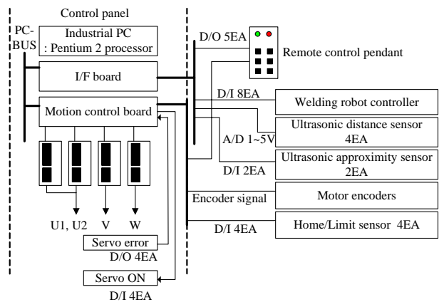
Fig. 9. Hardware architecture.
