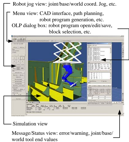
Fig. 2. The structure of the developed PC-based OLP.
