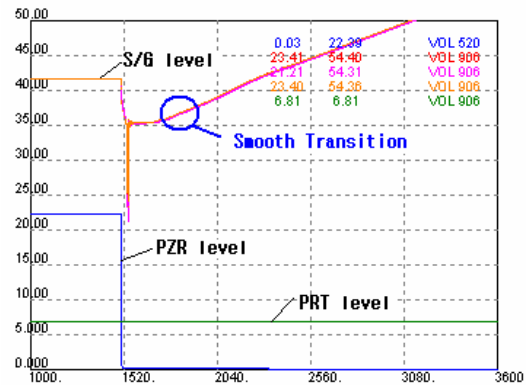
Figure 4. Water levels of the improved ARTS during 7 % LOCA simulation
