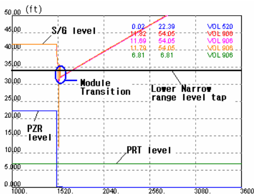
Figure 1. Water levels of the original ARTS during 25 % LOCA simulation
