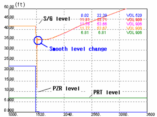
Figure 2. Water levels of the improved ARTS during 25 % LOCA simulation
