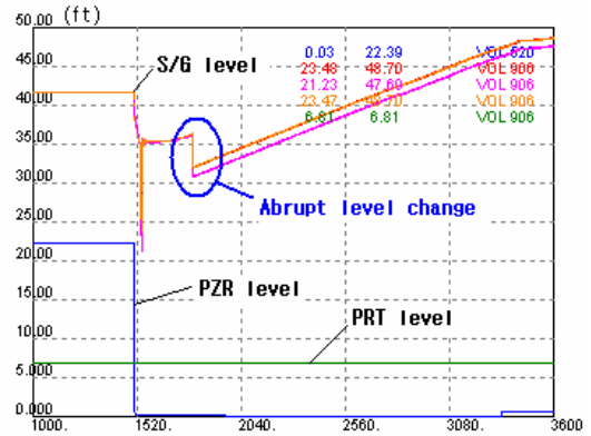
Figure 3. Water levels of the original ARTS during 7 % LOCA simulation
