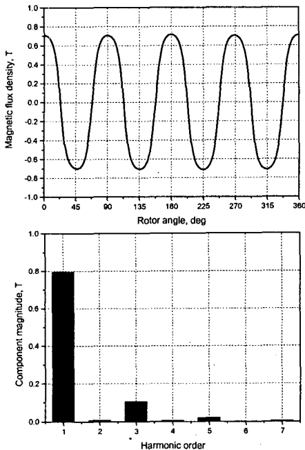
Fig. 5 Flux density distributed in the air-gap
