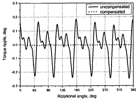
Fig. 6 Torque ripple compensation
