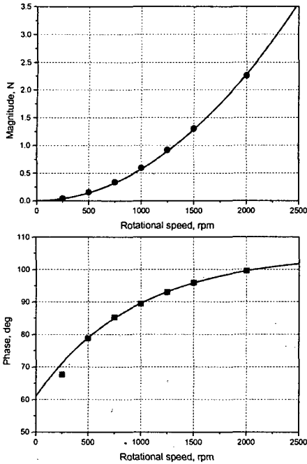
Fig. 11 Estimated unbalance force compensation vector
