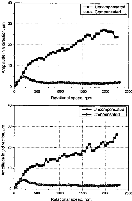
Fig. 12 Attenuation of radial vibration under the compensation
