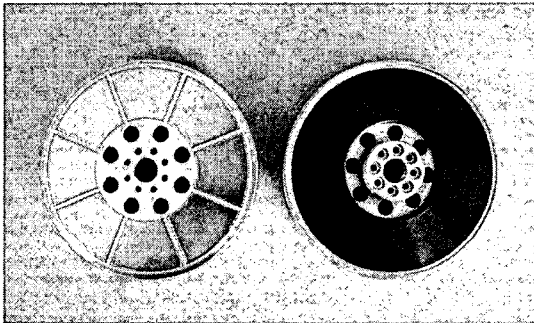
Fig 4 Rotor disks with 8 permanent magnets
