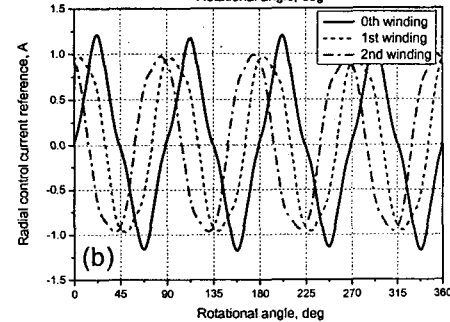
Fig. 8 Radial control current references for (a) x or (b) y directional force
