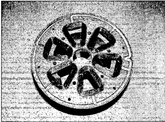
Fig 3 Stator with 6 concentrated windings
