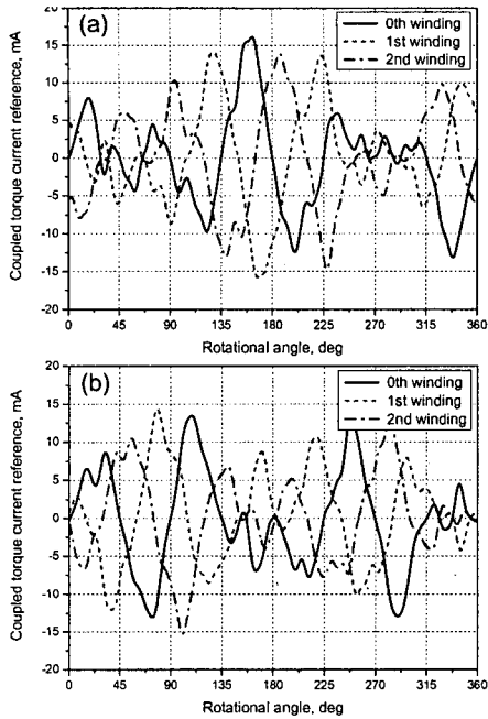
Fig. 9 Coupled torque current references for (a) x or (b) y directional force
