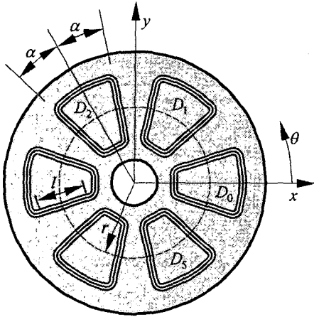
Fig. 1 Coordinates and winding distribution
