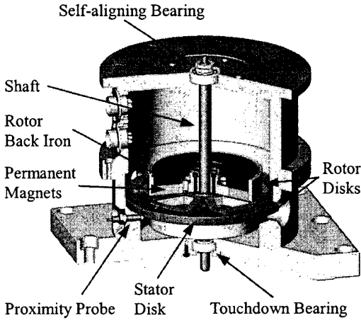
Fig. 2 Cutaway view of experimental setup
