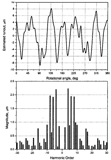
Fig. 10 Estimated runout profile and the directional spectrum
