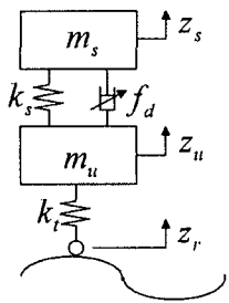
Fig. 7 Quarter car simulation model of semi-active suspension
