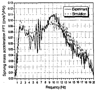
Fig. 11 Acceleration response of sprung mass
