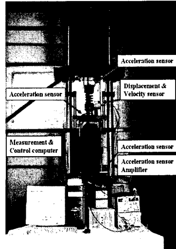
Fig. 8 Quarter car simulator
