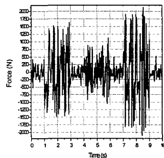
Fig. 4 Damping force for random displacement with current
