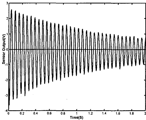
Fig.5 Free Vibration Response
