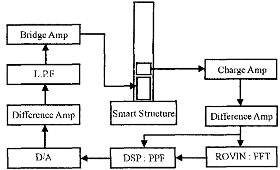
Fig.1 Control System
