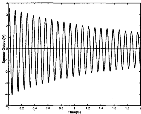
Fig. 6 Free Vibration Response with Added Mass
