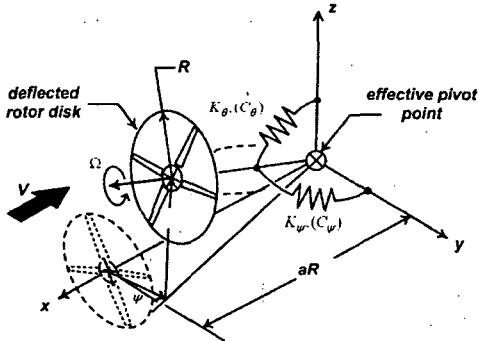
Fig. 2 Schematic view of 2-DOF rotor-nacelle dynamic system
