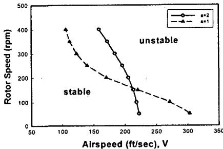
Fig. 12 Effect of airspeed and rotor speed for stable
