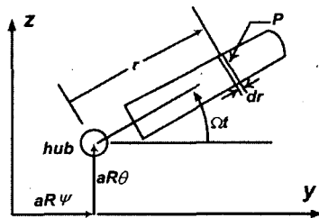
Fig. 3 Front view geometry of deflected hub and radially located typical section
