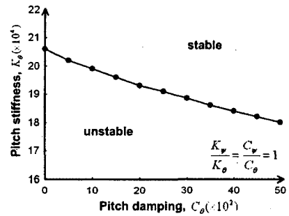
Fig. 10 Effect of pitch damping for whirl flutter stability
