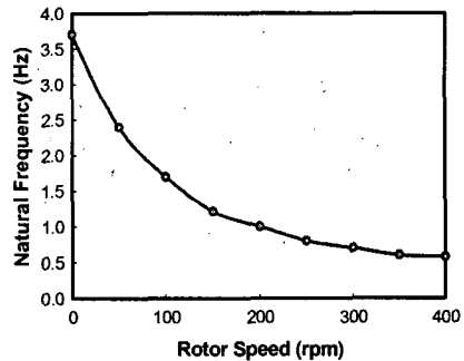
Fig. 6 Variation of natural frequency for different rotor speeds
