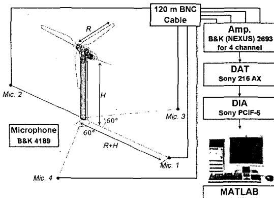
Fig. 1 Measurement locations and devices for acoustic quantities
