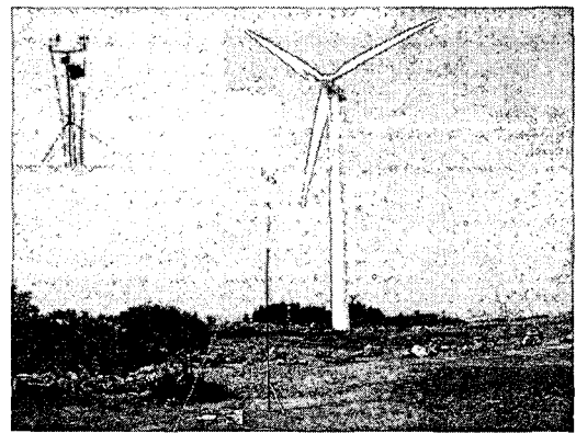
Fig. 2 Mobile meteorological mast at Hangwon
