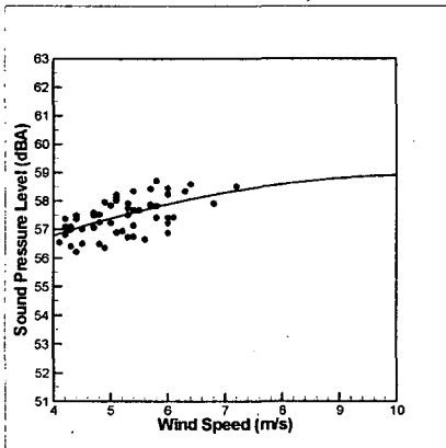
Fig. 4 Equivalent continuous sound pressure level of WTG (660 kW) at Hangwon (Regression curve: 53.4 + 1.03V - 0.047V^2 )
