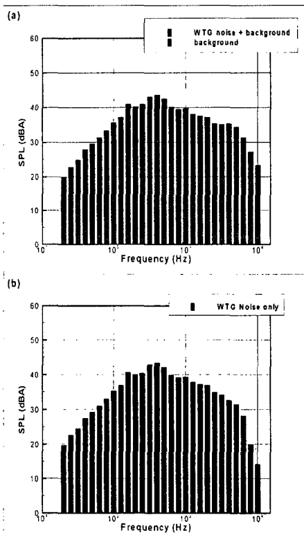
Fig. 6 Average one-third octave band of noise emission ( v=7m/s ) from 1.5MW WTG at Yongdang
