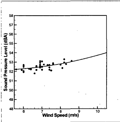
Fig. 3 Equivalent continuous sound pressure level of WTG (1.5 MW) at Youndang (Regression Curve: 5.30 - 0.40V + 0.047V^2 )
