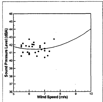
Fig. 5 ECSPL of background noise at Youndang
