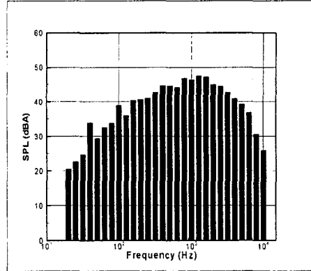
Fig. 7 Average one-third octave band of noise emission ( v=7m/s ) from 1.5MW WTG at Hangwon
