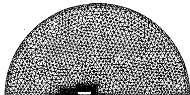
(a) Finite element modeling with fluid
