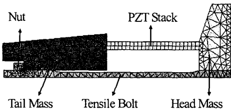
Fig. 1 Finite element model of Tonpiz type transducer
