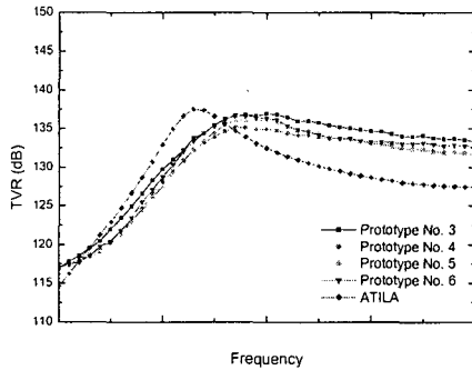
Fig. 5 Characteristic of transmitting voltage response (Major frequency span : 1 kHz)
