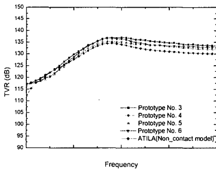
Fig. 6 Characteristic of transmitting voltage response of modified model (Major frequency span : 1 kHz)
