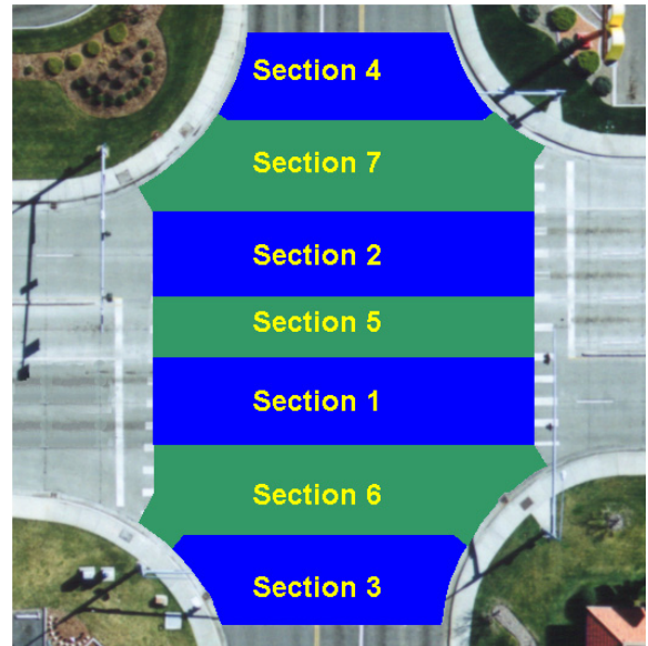
Figure 4. Concrete placement in interim Sections
