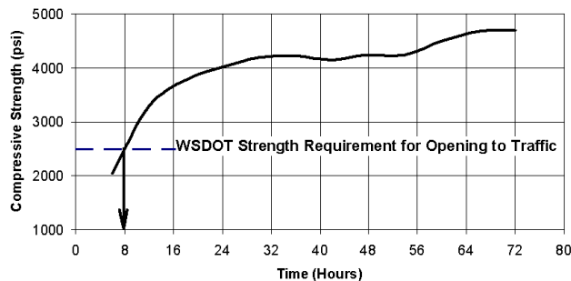
Figure 2. Compressive strength gain vs. time
