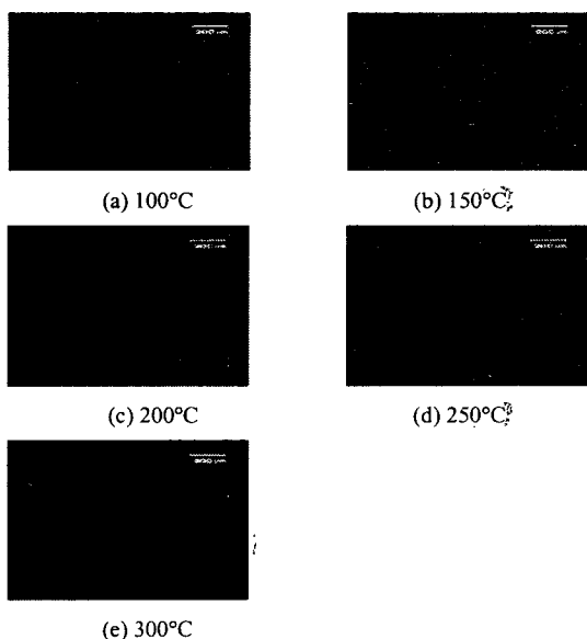
Fig. 4. Microphotographs of ion beam aligned LC cell on the SiC thin film for 10 min as a function of annealing temperature (in cross Nicols).
