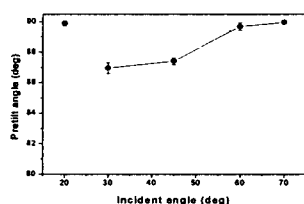
Fig. 3. Generation of pretilt angles in NLC with IB exposure on the SiC thin film surfaces for 1 min as a function of incident angle
