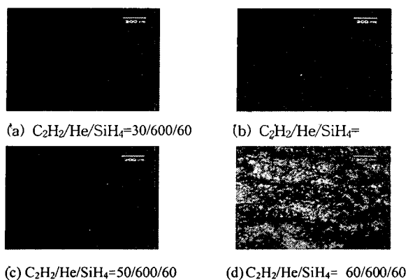
Fig. 2. Microphotographs of ion beam aligned LC cell on the four kinds of the SiC thin film (in crossed Nicols).
