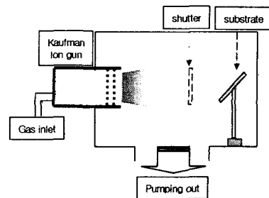
Figure 1. The ion beam (Kaufman type) exposure system.
